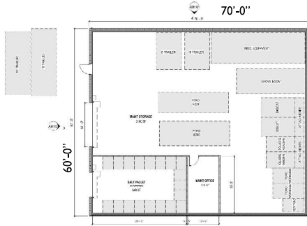
1 STORAGE BUILDING FLOOR PLAN
