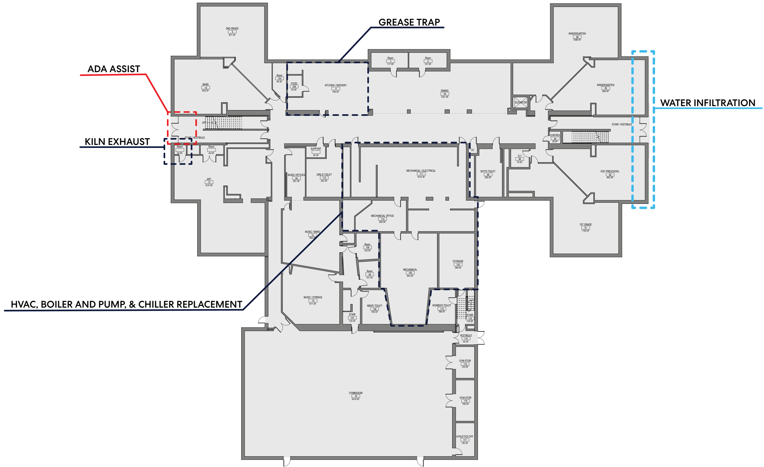
Existing Lower Level Floor Plan
