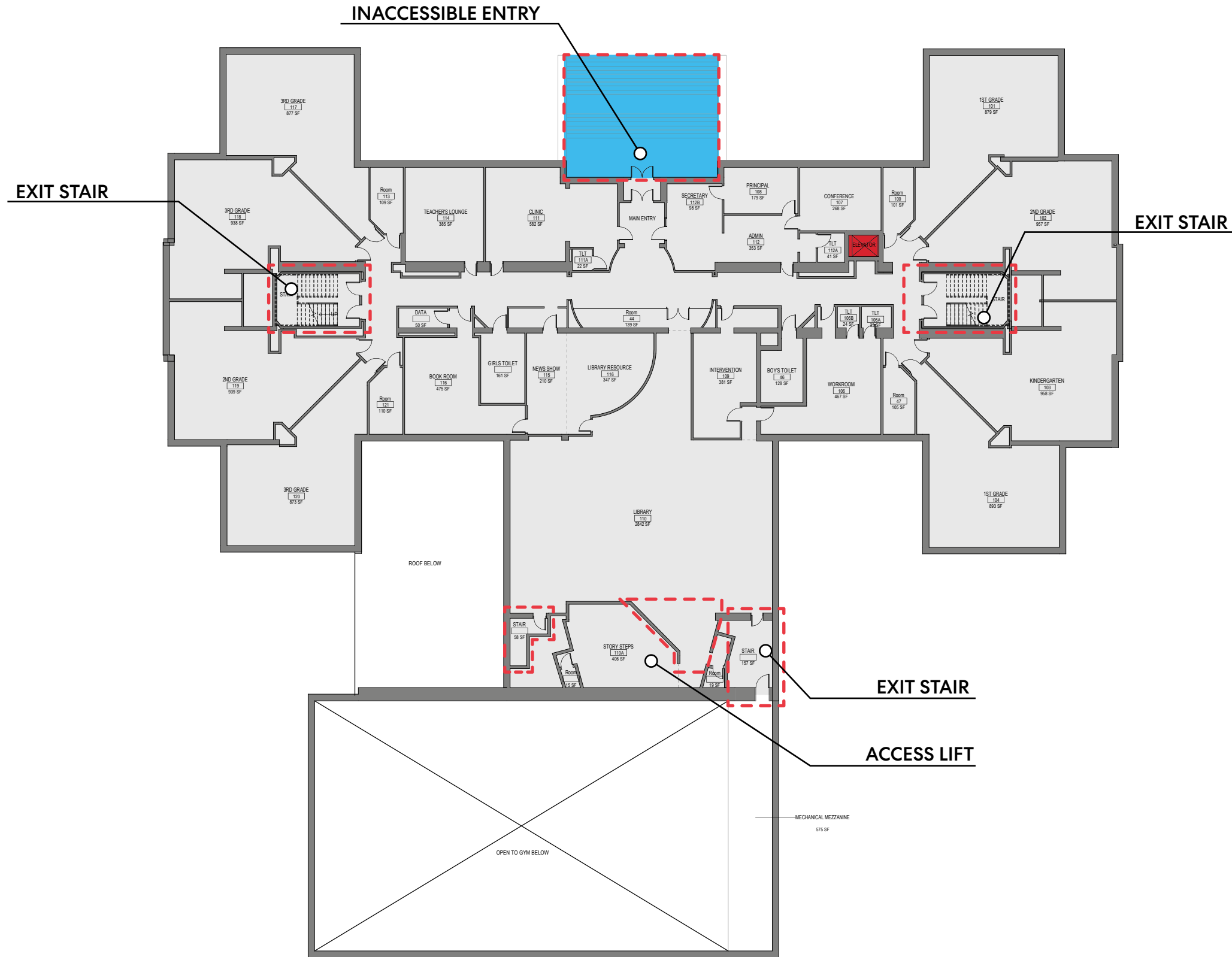
Existing First Floor Plan 0' 6' 12' 24' 48'
